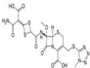
Figure 3. Core structure of cephamycins, cefoxitin, cefotetan and cefmetazole.
