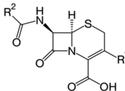
Cephalosporins(dihydrometathiazine ring)
