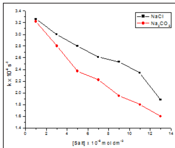
Fig.6 - Effect of Salt: [AA] = 3.8 x10 -5 mol dm -3 , TiO 2 = 300 mg/100 ml, Irradiation intensity=15 x10 3 lux, pH=9.0.
