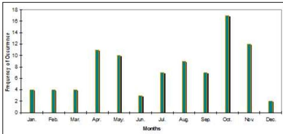
Figure 4 Shows the semi-annual variations of large storm events occurring during interval 1997-2007.
