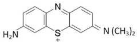
Fig. 1 - Structure of Azure A dye
