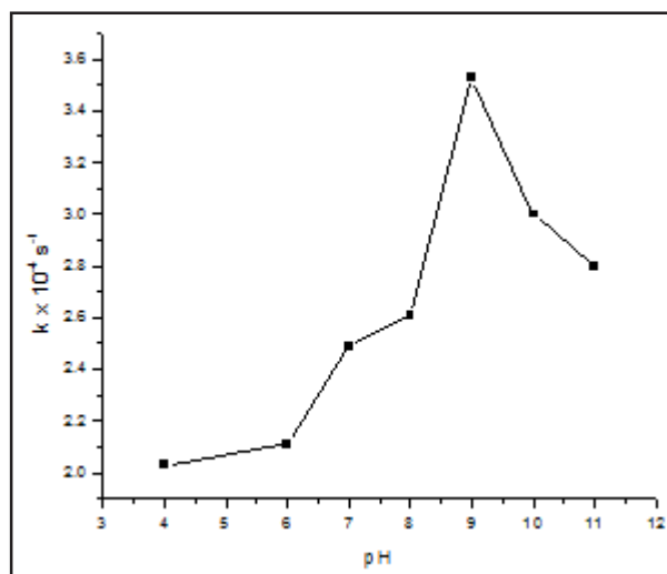
Fig.4 - Effect of pH :[AA] = 3.8 x 10 -5 mol dm -3 , TiO 2 = 300 mg/100 ml, Irradiation intensity=15 x 10 3 lux.
