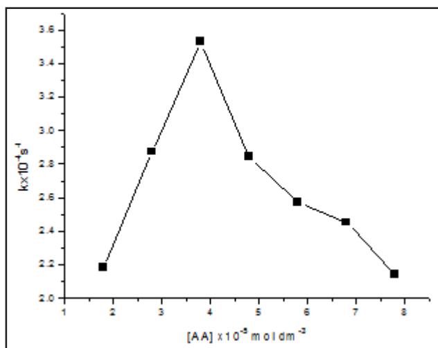
Fig.3: Effect of initial dye concentration: TiO 2 =300 mg/100 ml, Irradiation intensity=15 x10 3 lux, pH=9.0.
