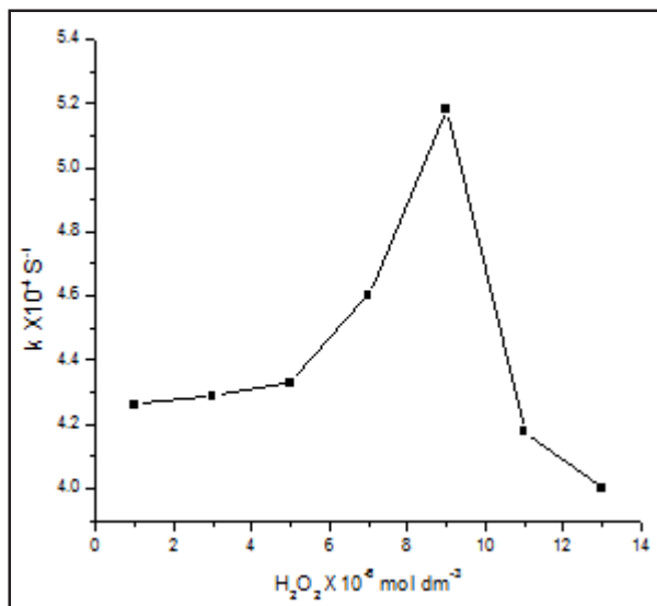
Fig.5 - Effect of hydrogen peroxide: [AA] = 3.8 \times 10^{-5} \text{ mol dm}^{-3} , TiO_2 = 300 \text{ mg}/100 \text{ ml} , Irradiation intensity = 15 \times 10^3 \text{ lux} , pH = 9.0 .
