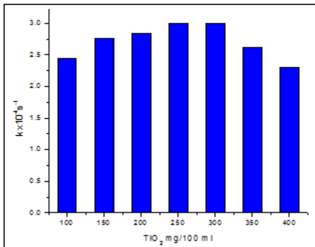
Fig.2 - Effect of TiO 2 loading: [AA] = 3.8 x 10 -5 mol dm -3 , Irradiation intensity=15 x 10 3 lux, pH=9.0.
