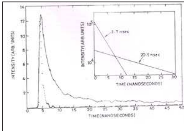
Fig.2 The time decay of the PL from 3 nm nanocrystalline ZnS: Mn 2+ . The last pulse is shown by dots as a reference. Inset: the time decay is separated into its exponential decay components (15).
