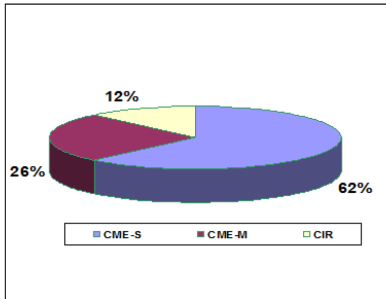
Figure 2. Shows the association of large geomagnetic storms with single/multiple CMEs and coronal holes
