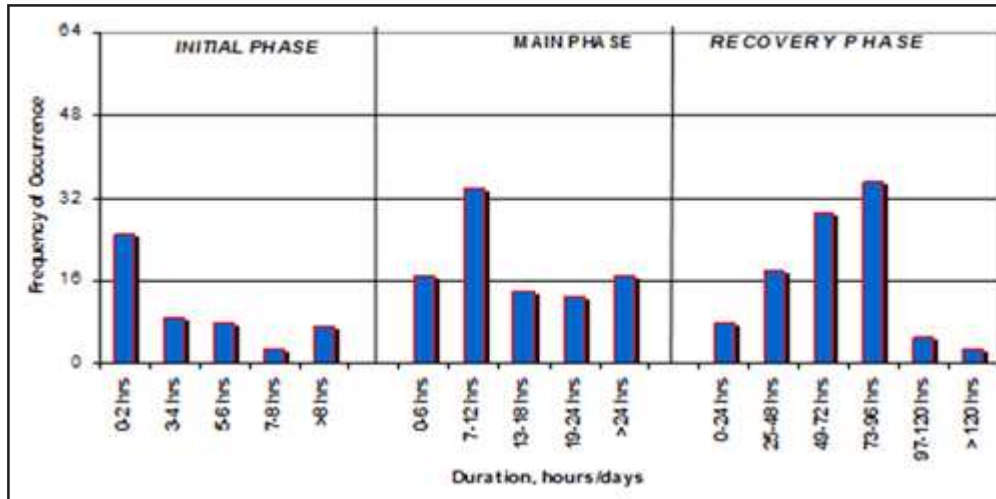
Figure 3. Frequency occurrence histogram show the initial, main and recovery phase duration for selected 90 large geomagnetic storms in above given specific range, observed during 1997-2007.
