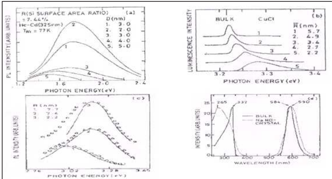
Fig. 1(a) PL spectra of (a) Si nanocrystals (ref.(6)), (b) CuCl nanocrystals (8), (c) ZnSe films deposited on quartz at 20 Pa and at different substrate temperature (9), and (d) Luminescence and excitation spectra of ZnS:Mn 2+ at room temperature. Solid line-bulk phosphors, dashed line-nanocrystals (10).
