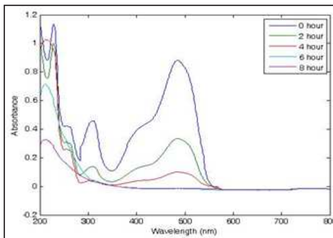
Fig.7 -Time dependent UV- visible absorption spectra depicting decolorization and complete degradation of Azure A using TiO_2 .
