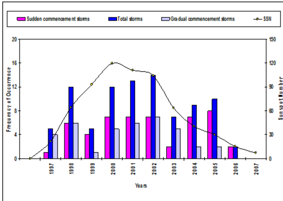
Figure 1. Shows the yearly occurrence of sudden commencement storm, total number of large geomagnetic storms and gradual commencement storm and their association with 11-year sunspot cycle, observed during 1997-2007 that covers solar cycle 23.
