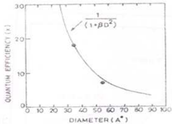
Fig. 3 Variation of luminescence quantum efficiency of ZnS: Mn 2+ nanocrystals as a function of the diameter. The solid line represents the equation \frac{1}{1+\beta D^2} (11).
