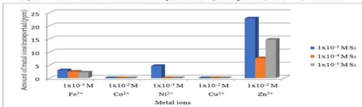
Figure 8 Amount of metal ions transported using ionophore in 24 hrs.
