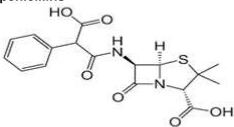
Figure 5. Structure of carboxypenicillins
