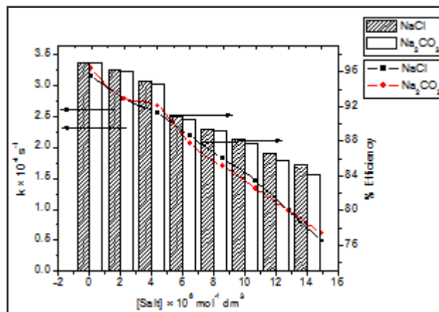
Fig. 1: Effect of Salt NaCl and Na_2CO_3
