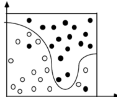
Fig. 1(c) Fuzzification
