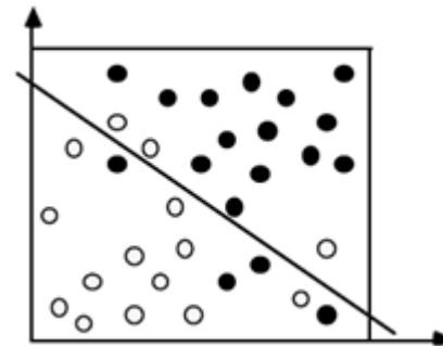
Fig. 1(b) Preprocession
