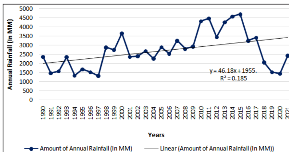
Fig. 2: Annual Trend of Rainfall in Balia Catchment(1990-2021)
