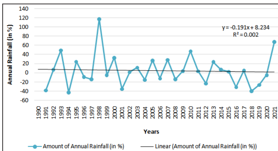
Fig. 3: Pattern of Annual Rainfall Change from (1990-2021) in Balia Catchment
