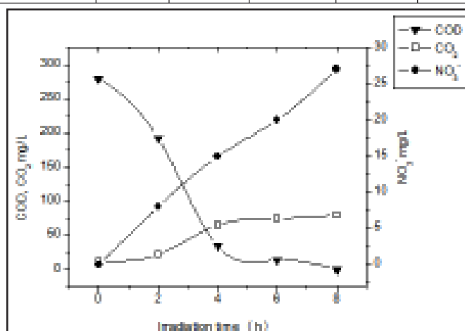
Fig. : COD and CO 2 measurements and formation of NO 3 - during photodegradation process of Methyl Green:
