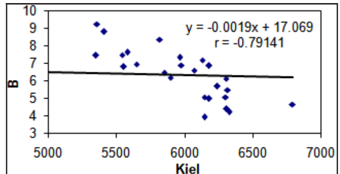
Fig 1.7:- Shows Correlation curve between yearly values of Inter planetary magnetic field (B) and Cosmic Ray Intensity (Kiel Neutron station) for the period 1986-2011.
