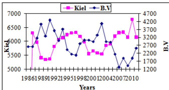
Fig 1.4:- Shows cross plot curve between yearly values of cosmic ray intensity (Kiel station) with B.V for the period 1986-2011.
