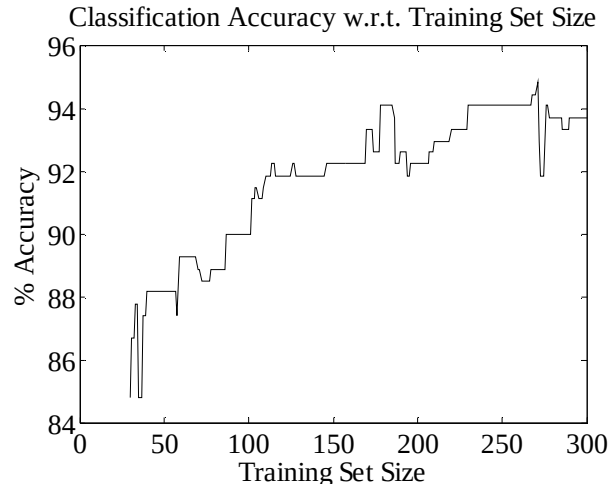
Fig. 6 Accuracy versus training set size of line outage-36
