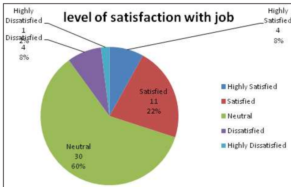
Graph 9
