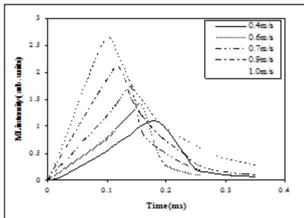
Fig.3 Time dependence of ML intensity of \text{Sr}(\text{VO}_3)_2:\text{Tb}(0.05 \text{ mol}\%) phosphors for different impact velocities ( \alpha -dose 1.395 kGy, mass of piston 0.4 kg)
