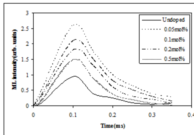
Fig.2 Time dependence of ML intensity of \text{Sr}(\text{VO}_3)_2:\text{Tb} phosphors for different concentration of dopant ( \gamma -dose 1.395 kGy, impact velocity 0.98 \text{ms}^{-1} , mass of piston 0.4 kg)
