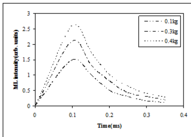
Fig.1 Time dependence of ML intensity of \text{Sr}(\text{VO}_3)_2:\text{Tb}(0.05 \text{ mol}\%) phosphors for different mass of piston ( \gamma -dose 1.395 kGy, impact velocity 0.98 \text{ms}^{-1} )
