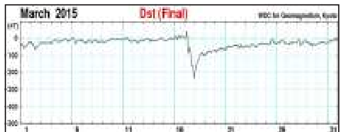
Graph (a) Dst value graph during storm month mar-2015
