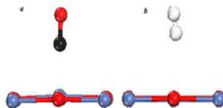
Figure 3-1: The used adsorption configurations for simulation. (a) CO adsorbate (b) H adsorbate above ceria
