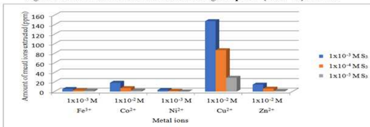
Figure 6 Amount of metal ions extracted using ionophore in 4 hrs.
