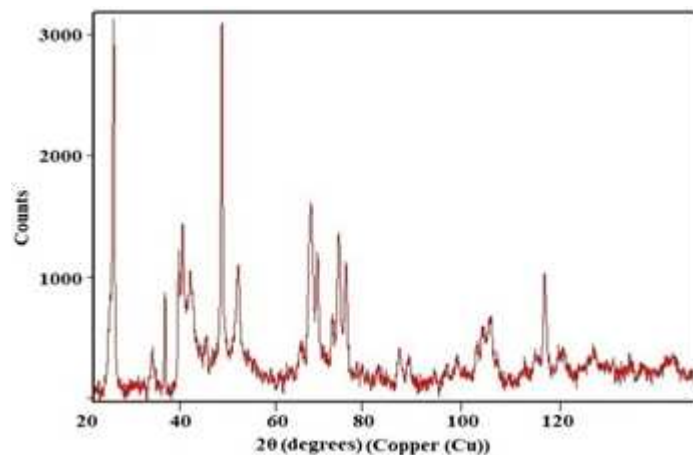
Fig. 1 XRD pattern of zero valent iron nanoparticles.
