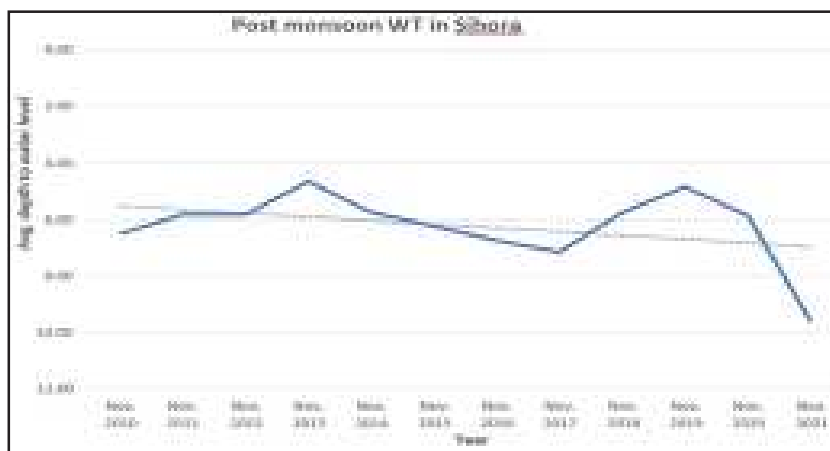
Fig. 14: Decadal trend of post monsoon water table in Sihora block
