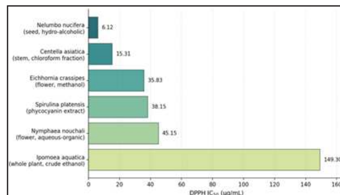
Figure 1: Comparative DPPH Radical-Scavenging Potency of Selected Aquatic Medicinal Plant Extracts
