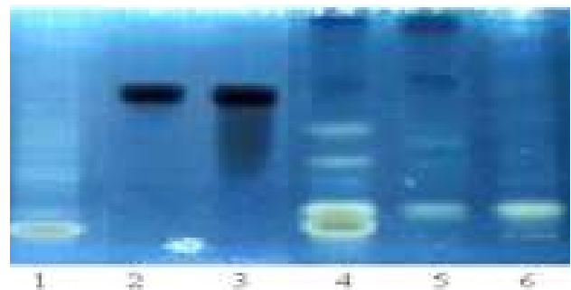
Fig. HPTLC profile of flavonoid finger prints of ethanol extract of selected medicinal plants using Rutin as a marker compound.
