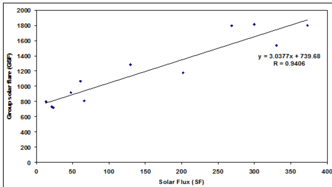
Figure 1. Shows the cross plot between yearly mean values of grouped solar flares and solar flux for the solar cycle 23.
