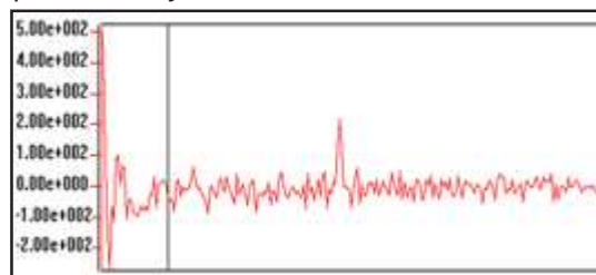
Fig-2: Cepstrum of the latter /a:/'
