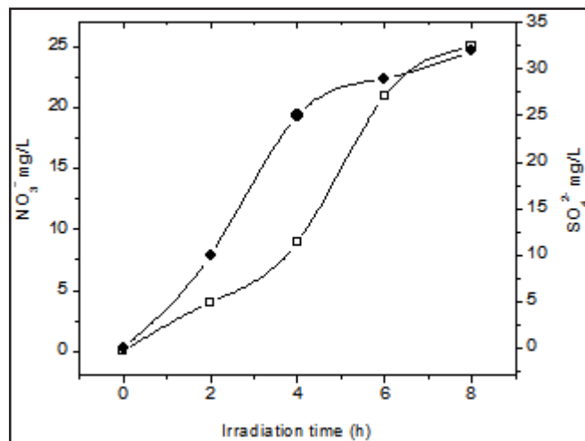
Fig. 2 Formation of \text{SO}_4^{2-} and \text{NO}_3^- during mineralization Azure A:
