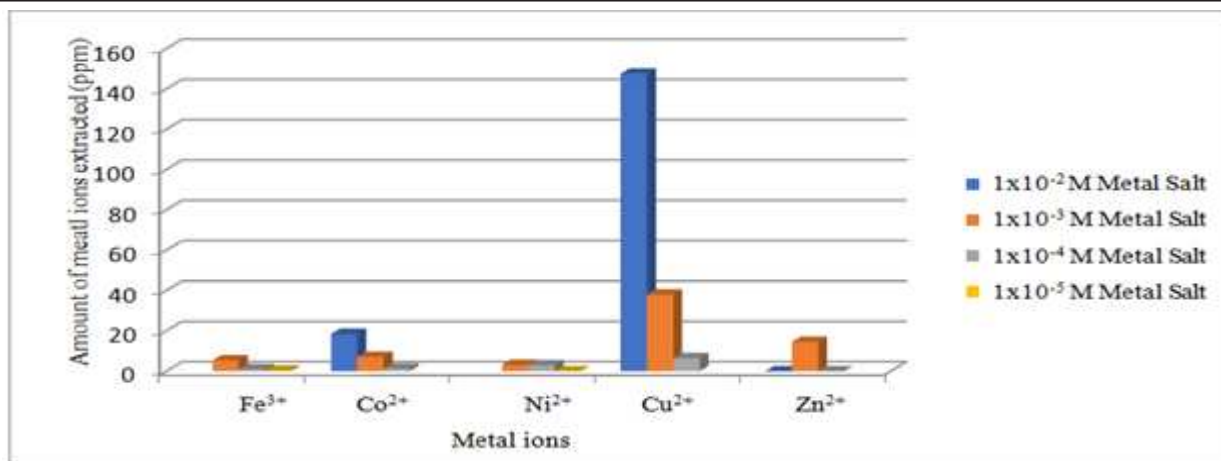
Figure 5 Amount of metal ions extracted using ionophore (1x10 -3 M) in 4 hrs.
