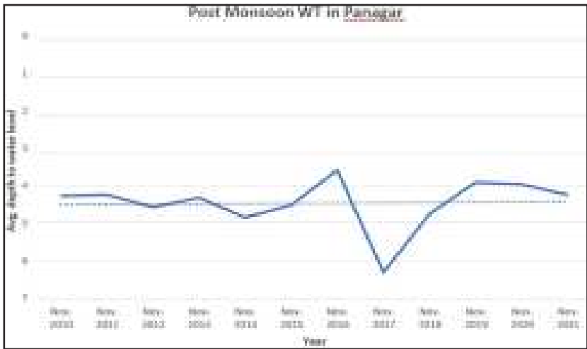
Fig 11: Decadal trend of post monsoon water table in Panagar block
