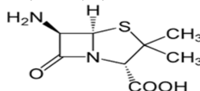
Figure 3. Structure of 6-APA: Amino group is acylated to R-CO-NH- group present in semisynthetic penicillin.
