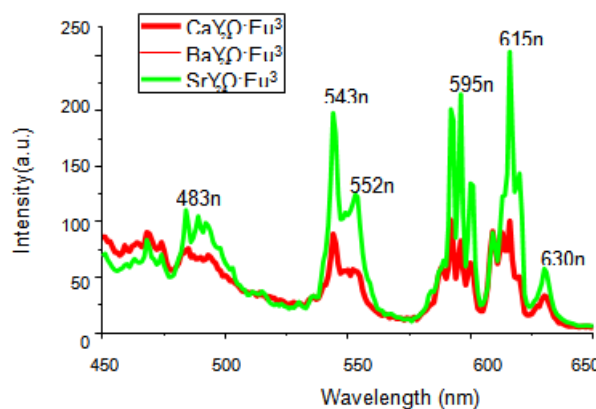
Figure 2 PL excitation spectra for \text{MY}_2\text{O}_4:\text{Eu}^{3+} phosphor
