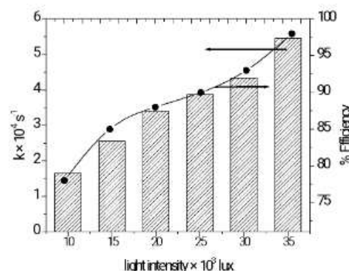
Fig.2: Effect of light intensity
